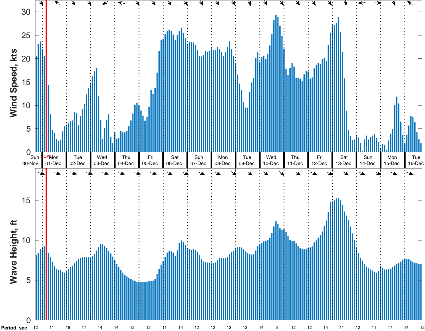
Wind & Wave Forecast for NDBC 46028 SWAN from 30-Nov-2025 17:00:00 to 16-Dec-2025 17:00:00
