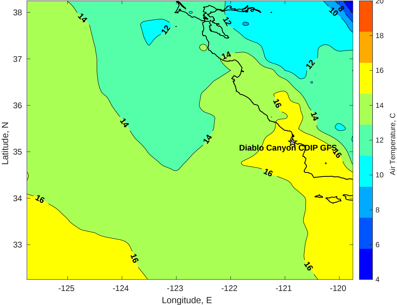
Air Temperature (C) for Diablo Canyon CDIP GFS at 02-Dec-2025
