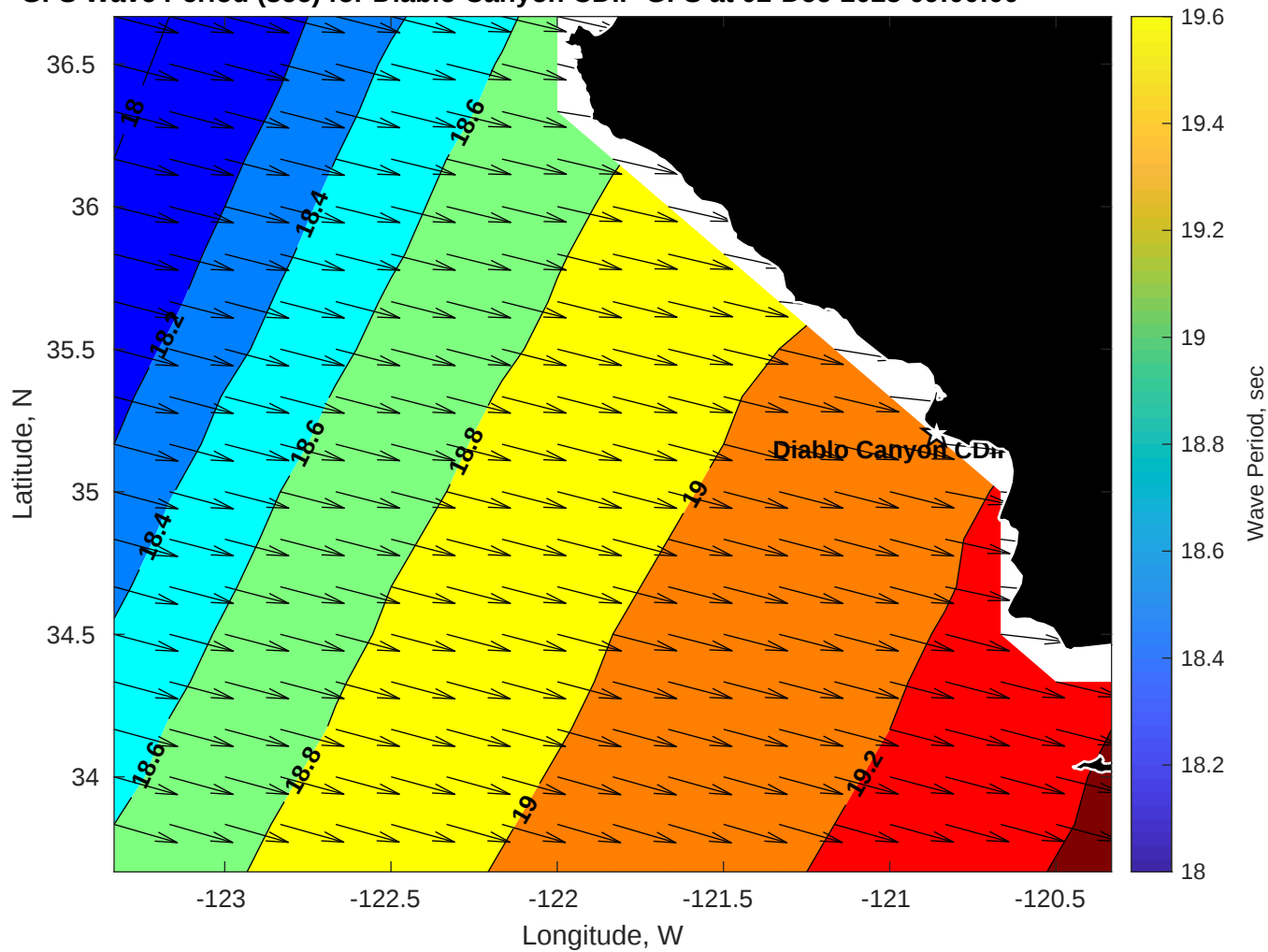
GFS Wave Period (sec) for Diablo Canyon CDIP GFS at 02-Dec-2025 09:00:00
