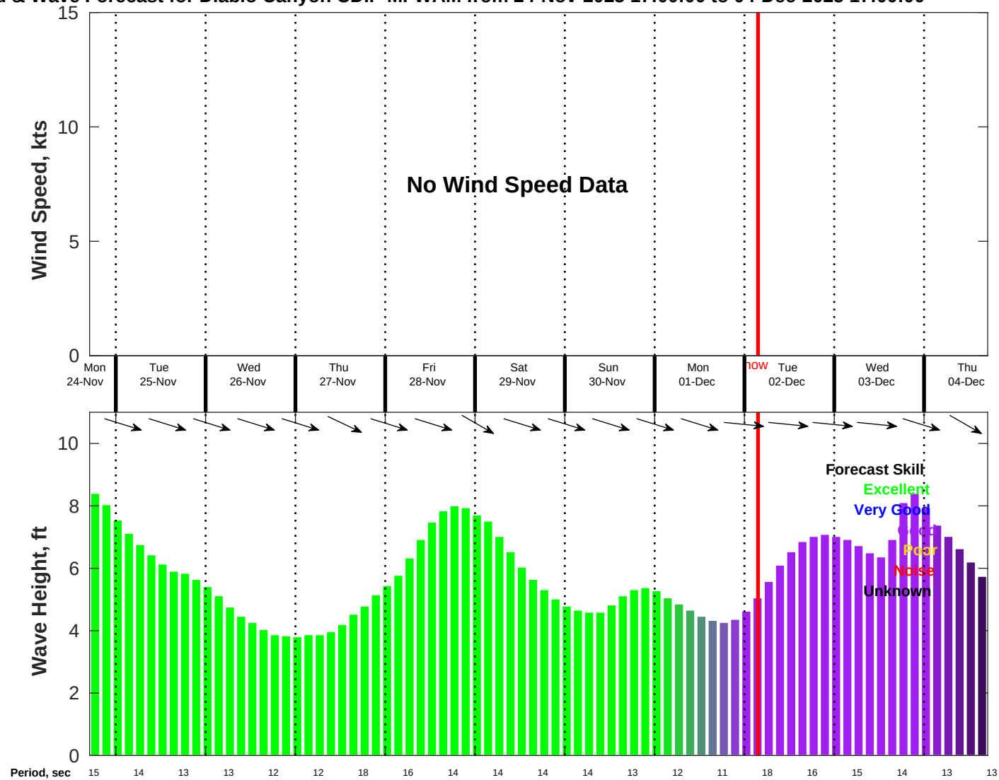
Wind & Wave Forecast for Diablo Canyon CDIP MFWAM from 24-Nov-2025 17:00:00 to 04-Dec-2025 17:00:00
