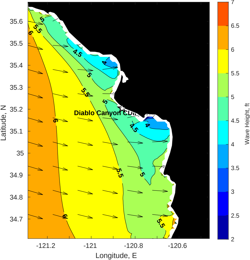
SWAN Wave Height (ft) for Diablo Canyon CDIP SWAN at 02-Dec-2025 10:00:00
