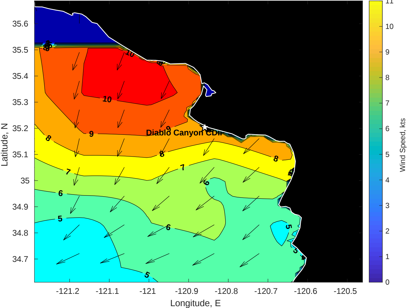
SWAN Winds (kts) for Diablo Canyon CDIP SWAN at 02-Dec-2025 10:00:00
