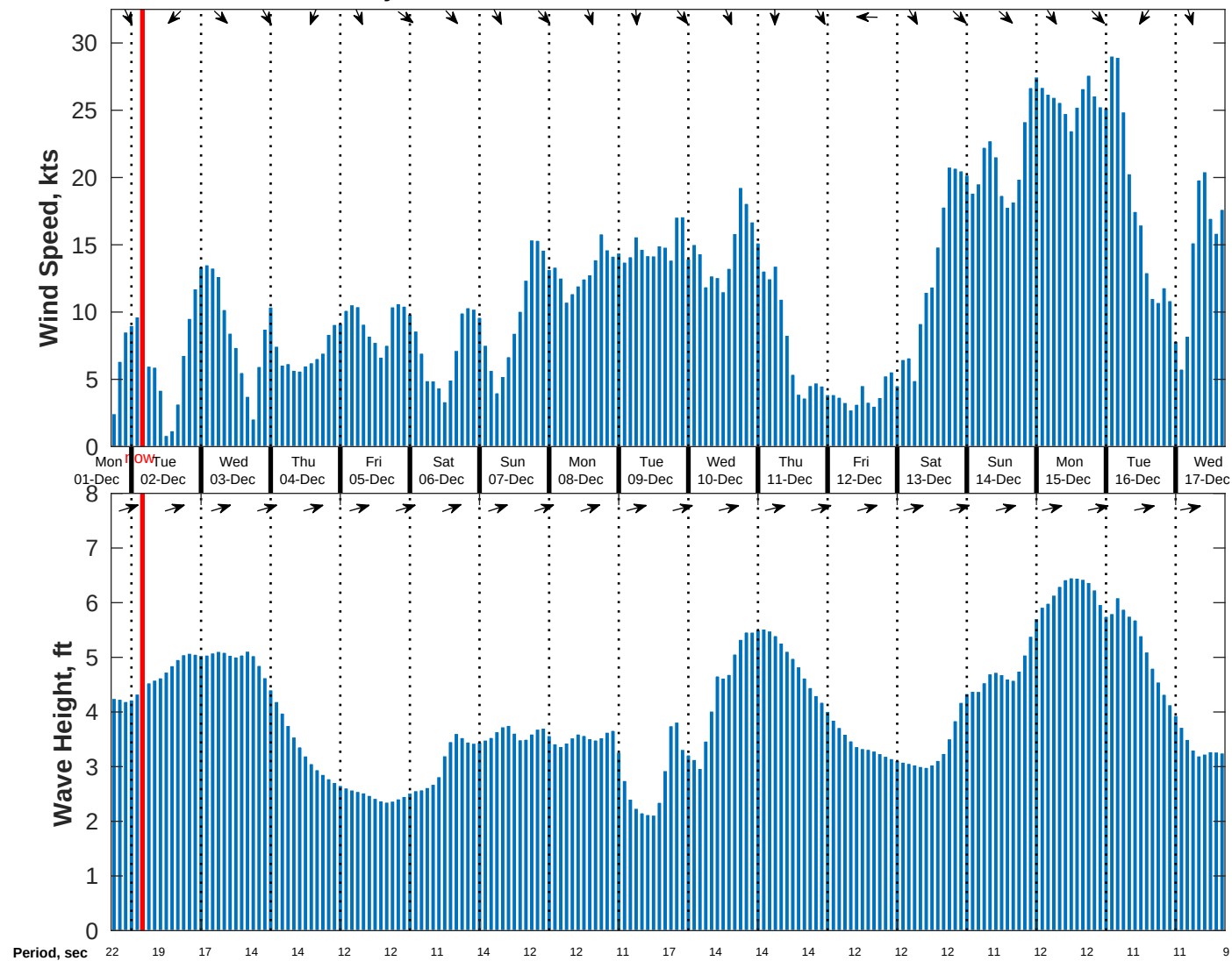
Wind & Wave Forecast for Diablo Canyon CDIP SWAN from 01-Dec-2025 17:00:00 to 17-Dec-2025 17:00:00
