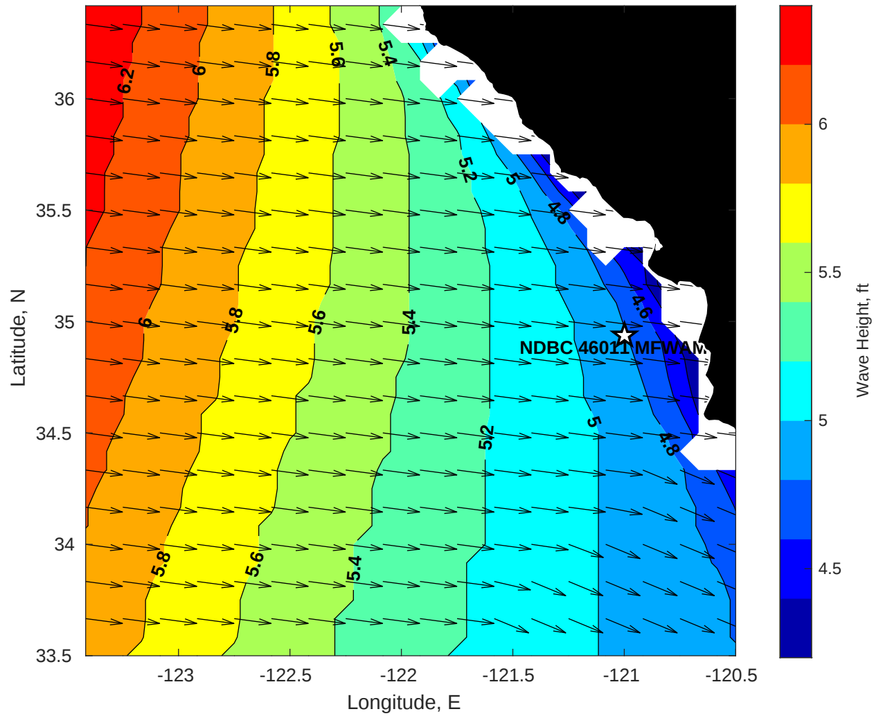
WAM Wave Height (ft) for NDBC 46011 MFWAM at 02-Dec-2025 09:00:00
