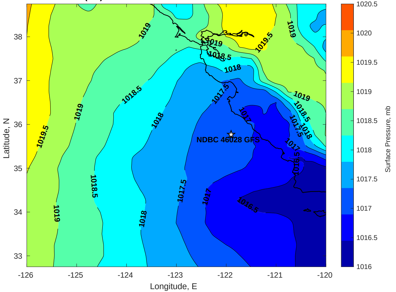
Surface Pressure (mb) for NDBC 46028 GFS at 02-Dec-2025 00:00:00
