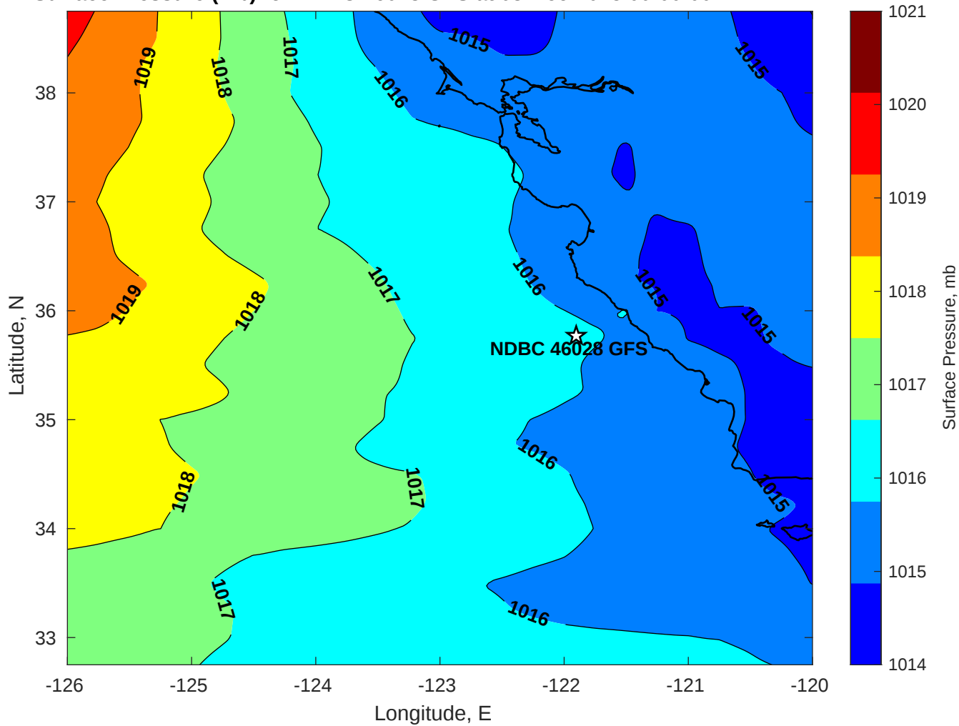
Surface Pressure (mb) for NDBC 46028 GFS at 03-Dec-2025 00:00:00
