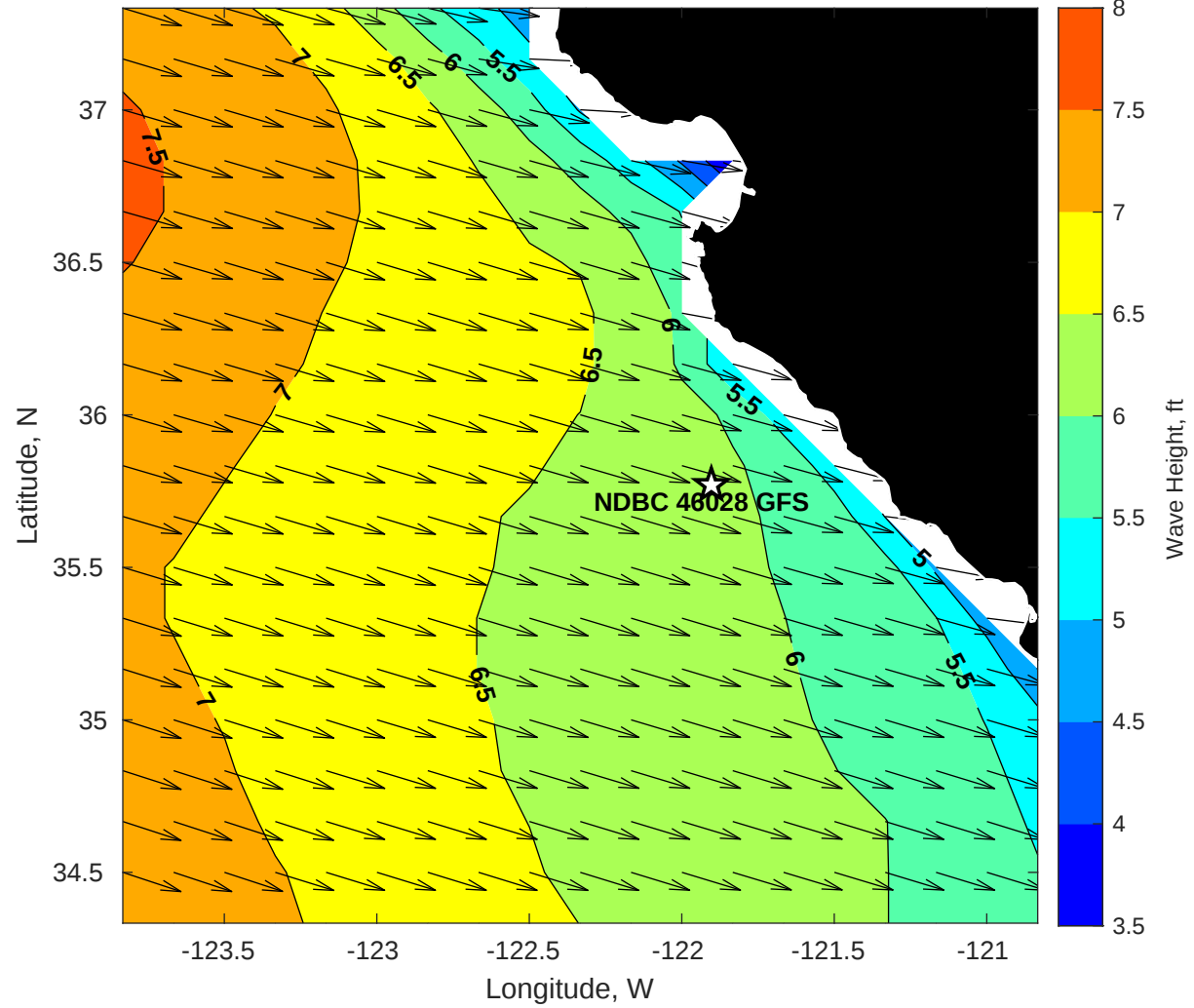
GFS Wave Height (ft) for NDBC 46028 GFS at 02-Dec-2025 09:00:00
