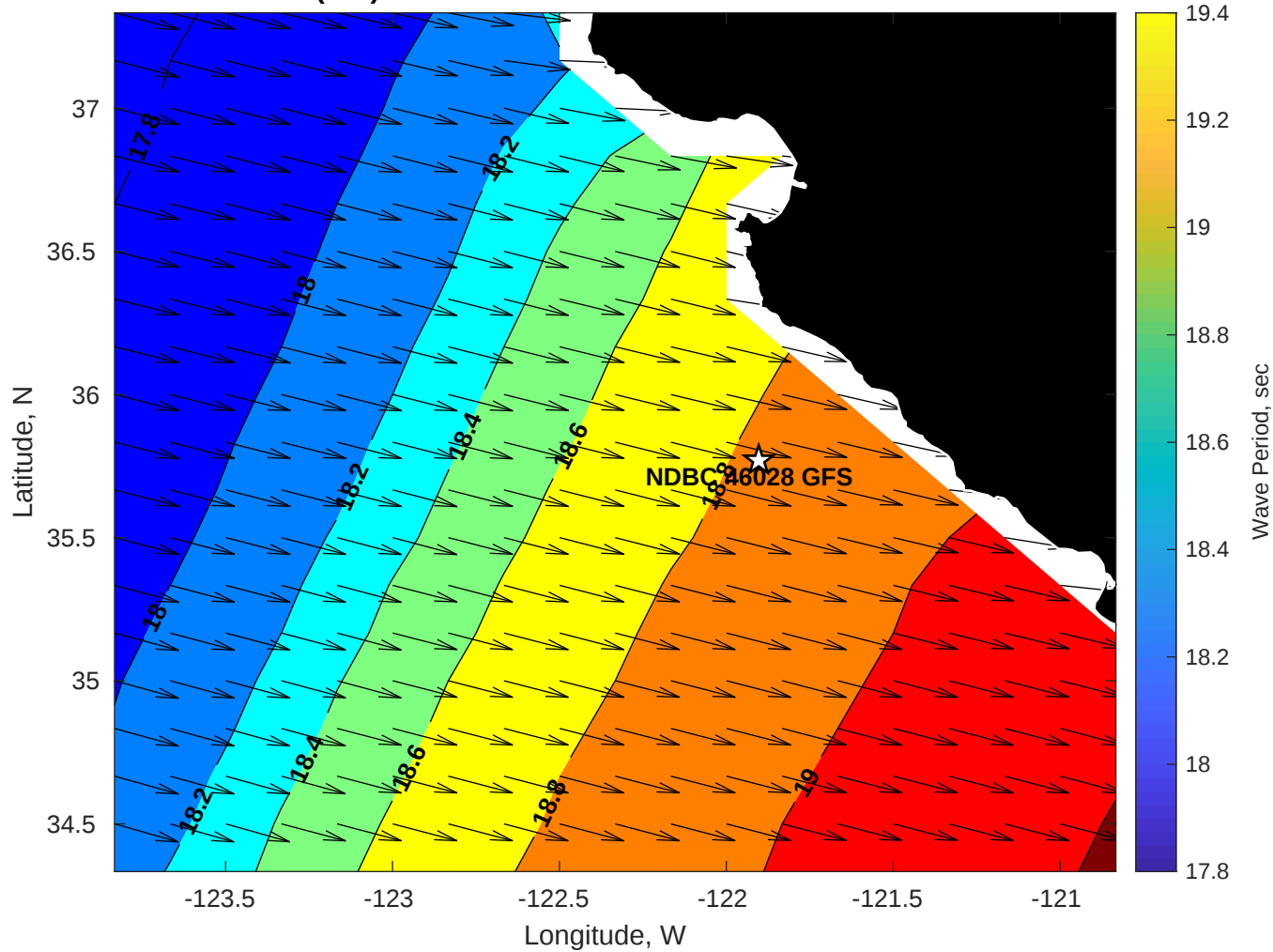
GFS Wave Period (sec) for NDBC 46028 GFS at 02-Dec-2025 09:00:00
