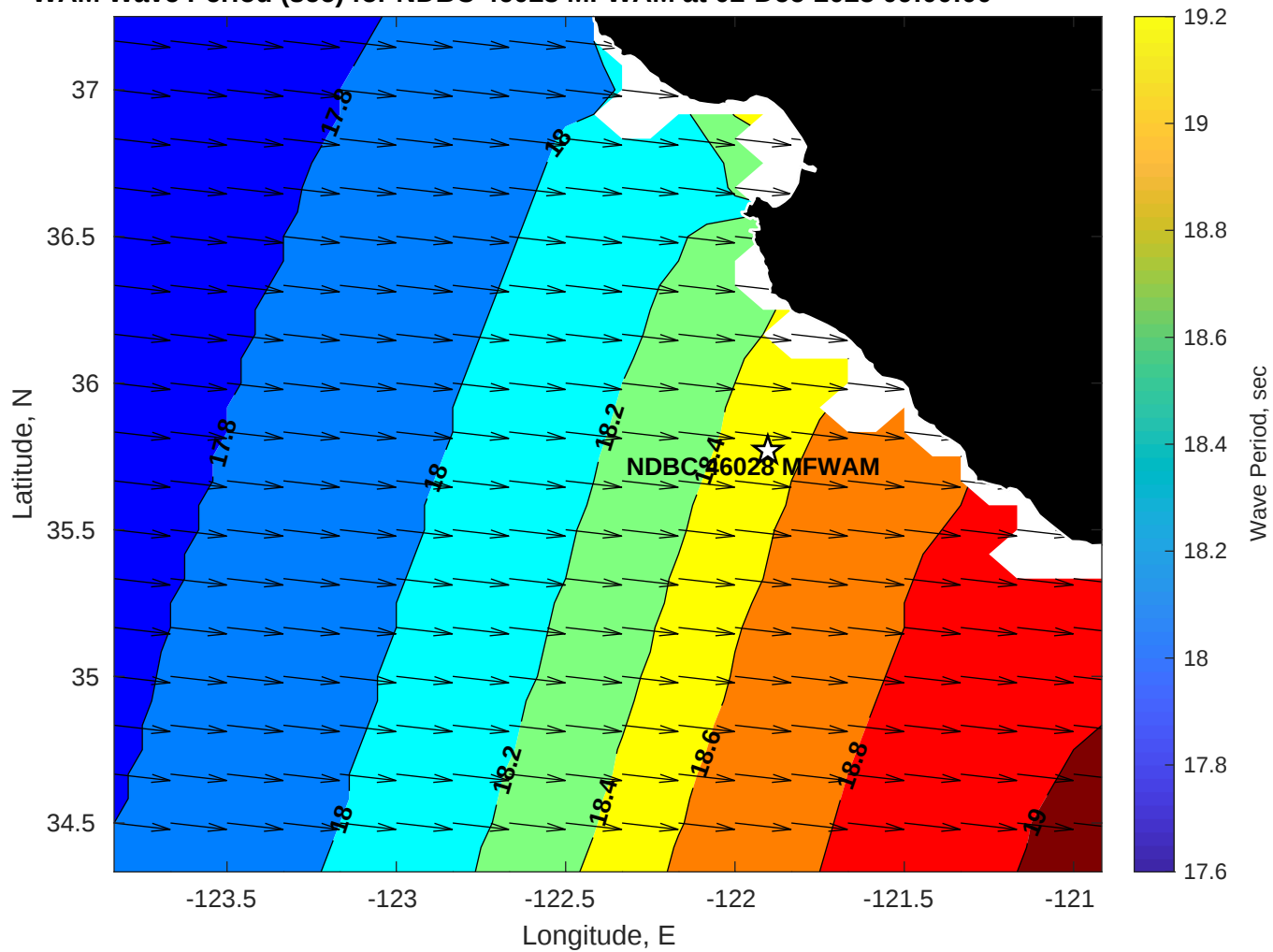
WAM Wave Period (sec) for NDBC 46028 MFWAM at 02-Dec-2025 09:00:00
