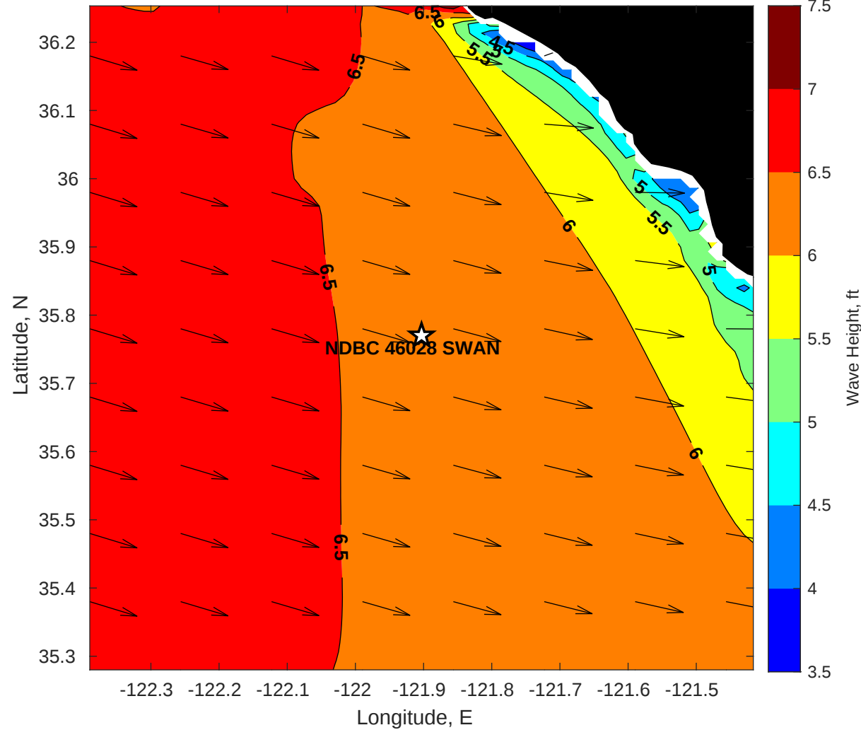
SWAN Wave Height (ft) for NDBC 46028 SWAN at 02-Dec-2025 10:00:00
