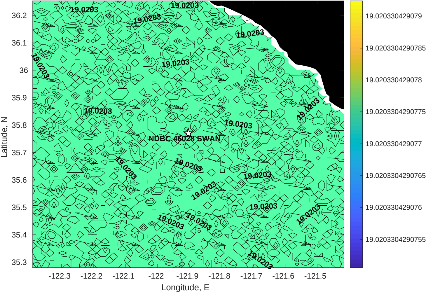
SWAN Wave Period (sec) for NDBC 46028 SWAN at 02-Dec-2025 10:00:00
