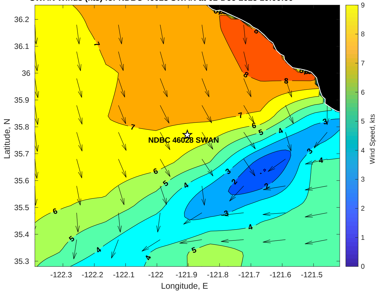
SWAN Winds (kts) for NDBC 46028 SWAN at 02-Dec-2025 10:00:00
