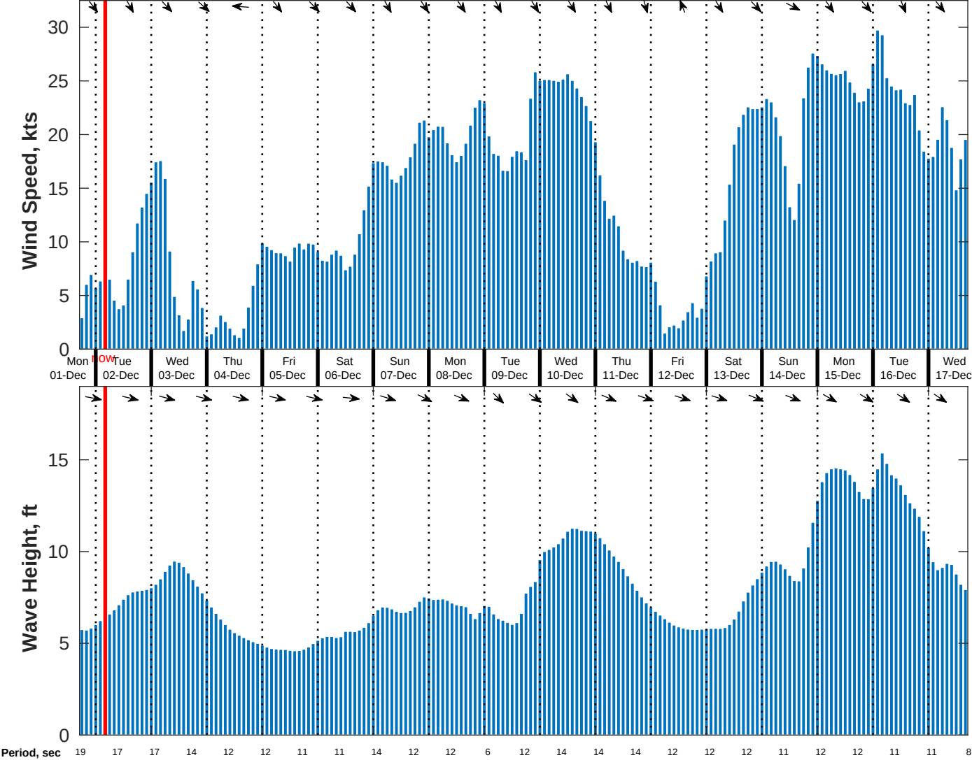
Wind & Wave Forecast for NDBC 46028 SWAN from 01-Dec-2025 17:00:00 to 17-Dec-2025 17:00:00
