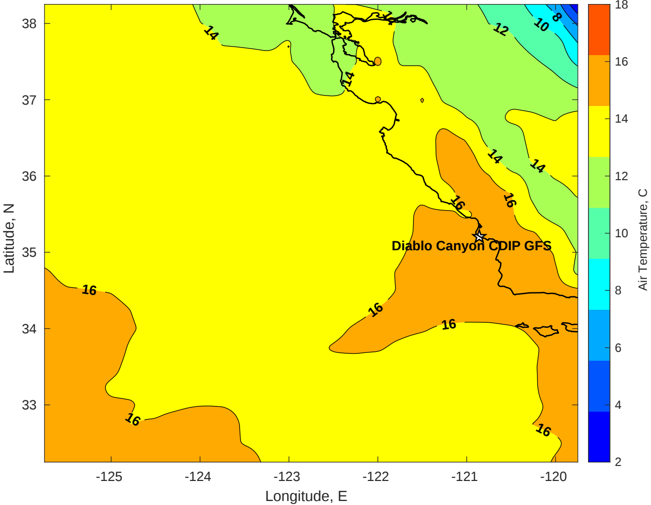
Air Temperature (C) for Diablo Canyon CDIP GFS at 03-Dec-2025
