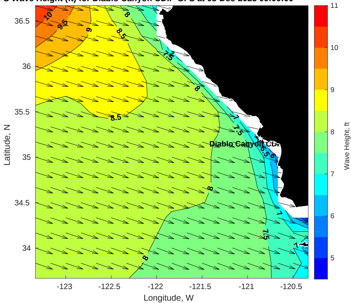
GFS Wave Height (ft) for Diablo Canyon CDIP GFS at 03-Dec-2025 09:00:00
