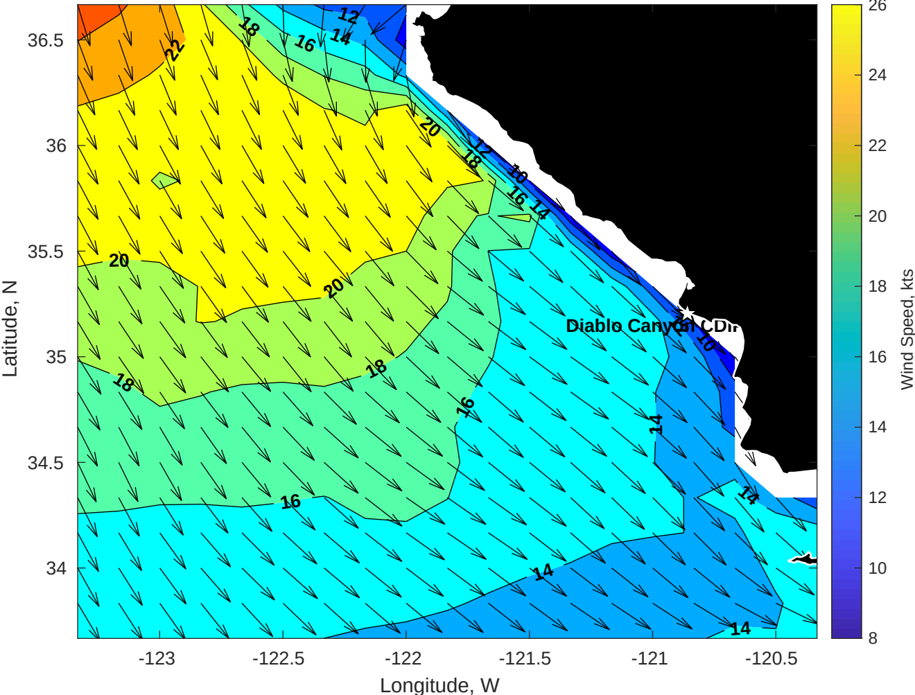
GFS Winds (kts) for Diablo Canyon CDIP GFS at 03-Dec-2025 09:00:00
