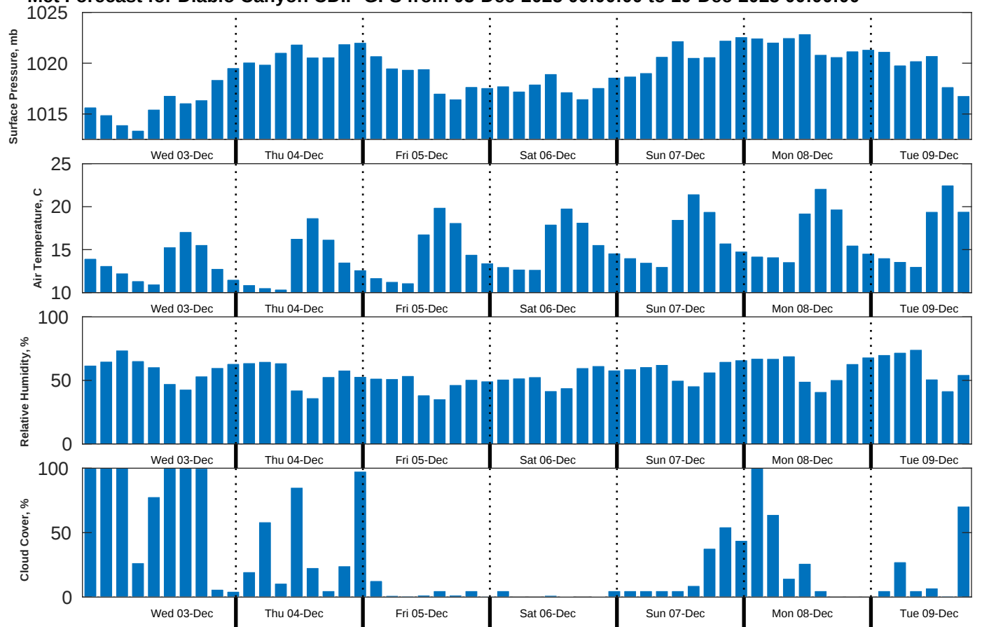
Met Forecast for Diablo Canyon CDIP GFS from 03-Dec-2025 00:00:00 to 10-Dec-2025 00:00:00
