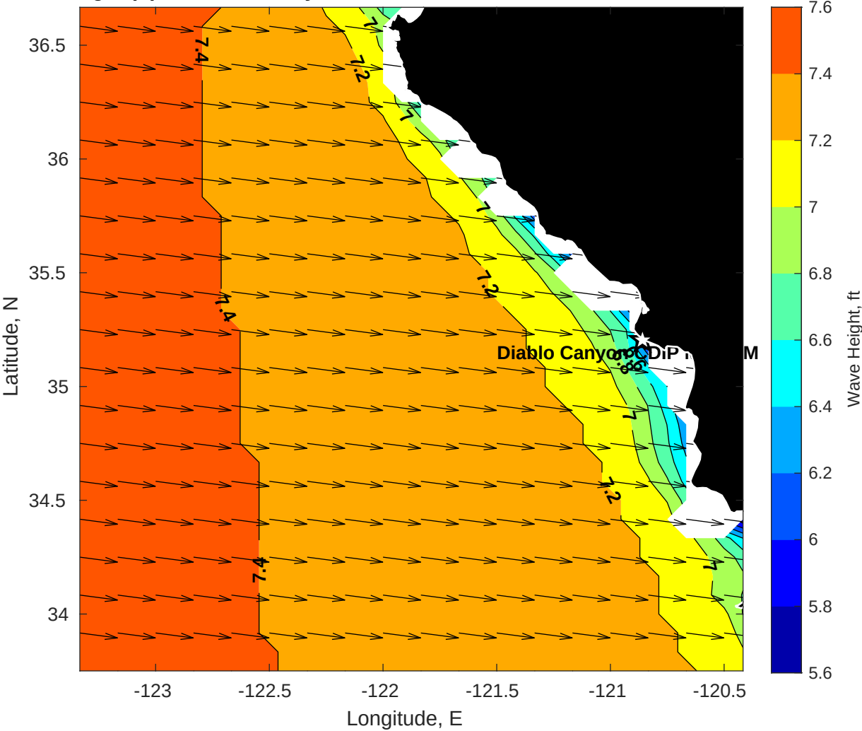
WAM Wave Height (ft) for Diablo Canyon CDIP MFWAM at 03-Dec-2025 09:00:00
