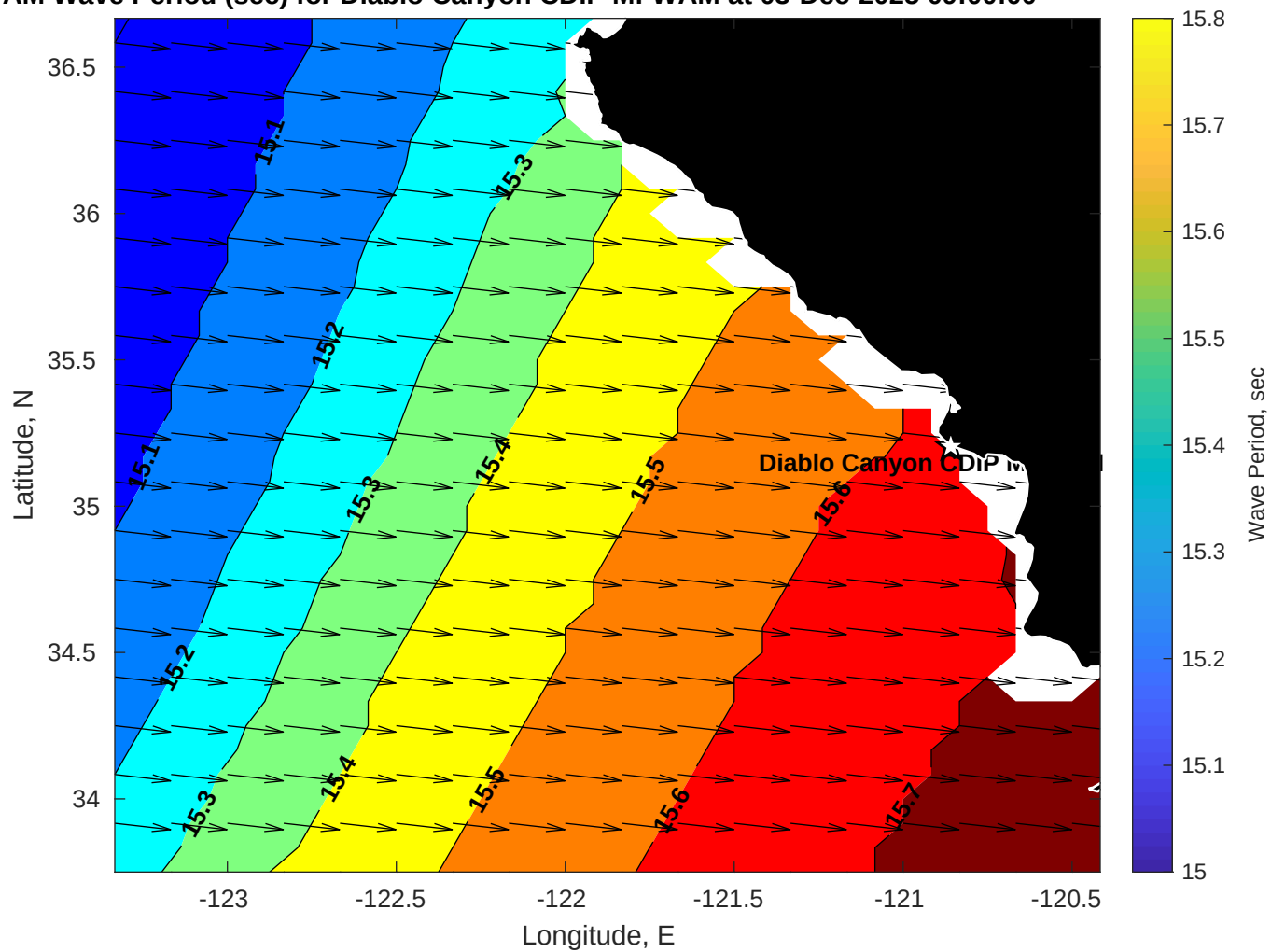
WAM Wave Period (sec) for Diablo Canyon CDIP MFWAM at 03-Dec-2025 09:00:00
