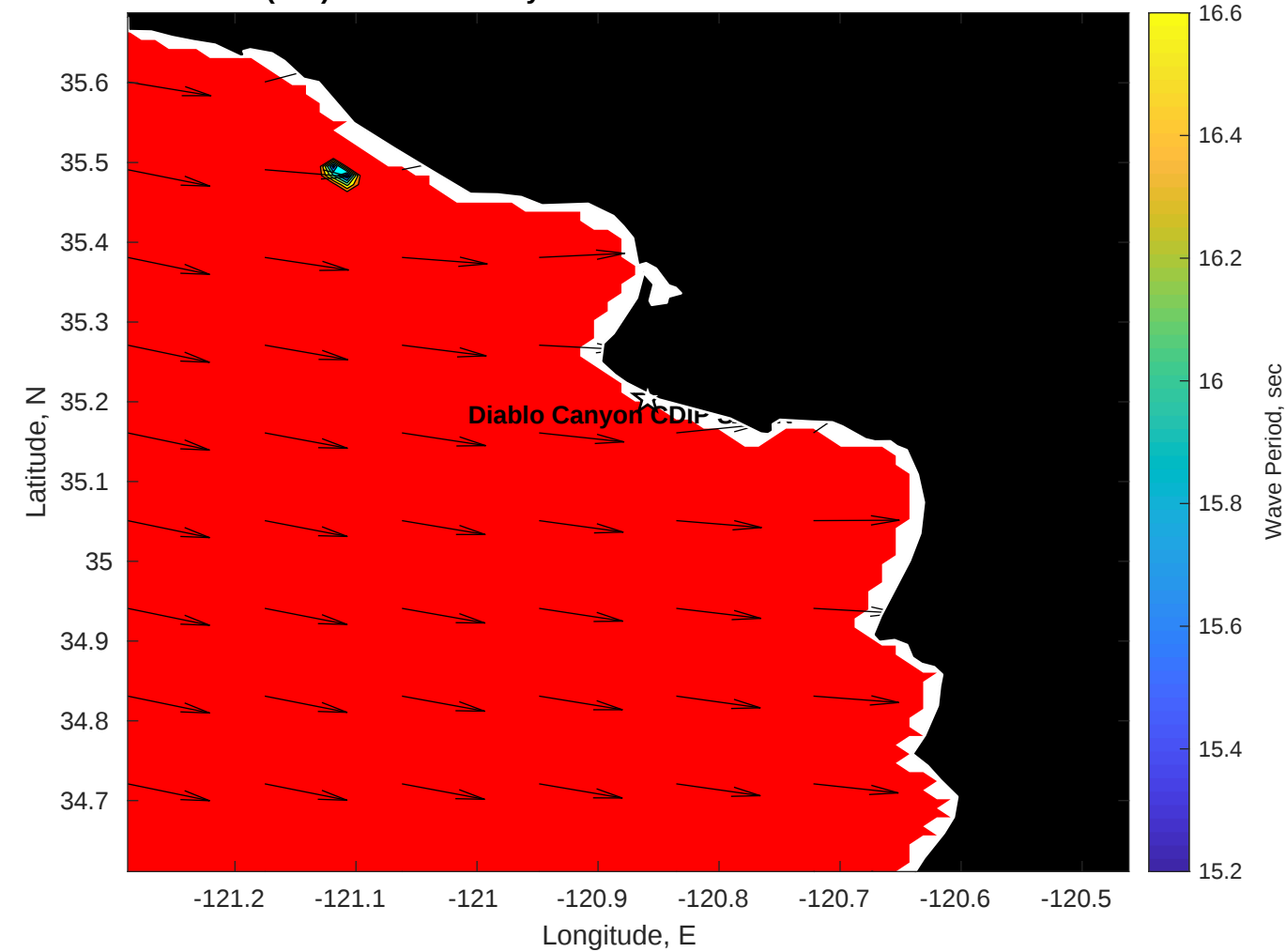
SWAN Wave Period (sec) for Diablo Canyon CDIP SWAN at 03-Dec-2025 10:00:00
