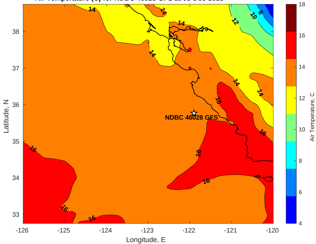
Air Temperature (C) for NDBC 46028 GFS at 03-Dec-2025
