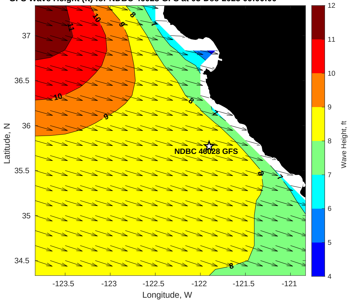
GFS Wave Height (ft) for NDBC 46028 GFS at 03-Dec-2025 09:00:00
