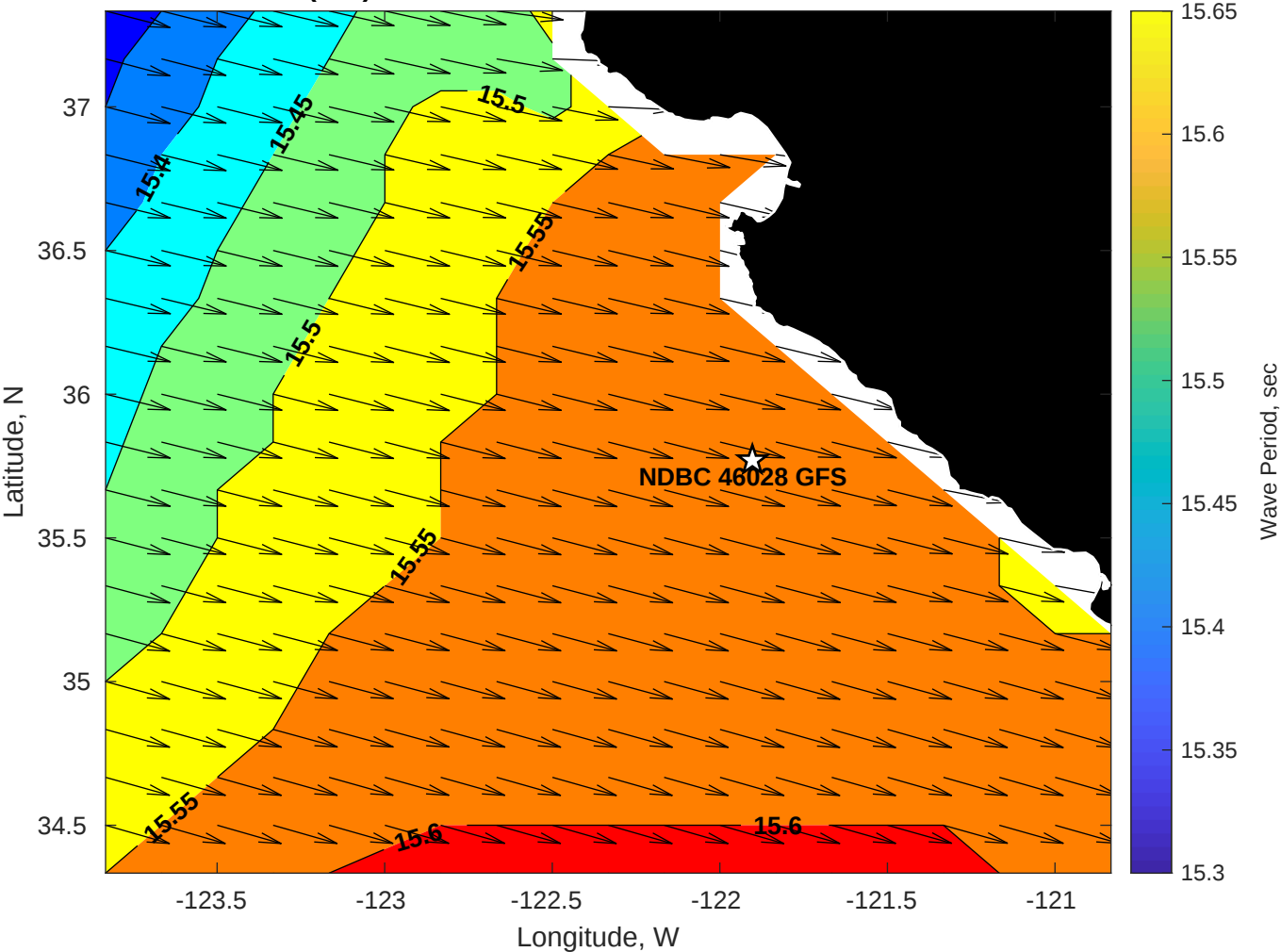
GFS Wave Period (sec) for NDBC 46028 GFS at 03-Dec-2025 09:00:00
