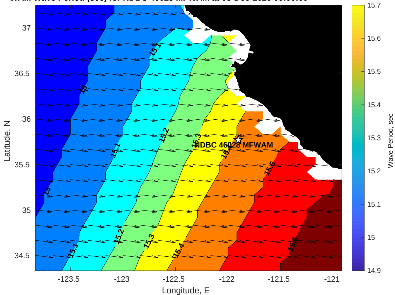
WAM Wave Period (sec) for NDBC 46028 MFWAM at 03-Dec-2025 09:00:00
