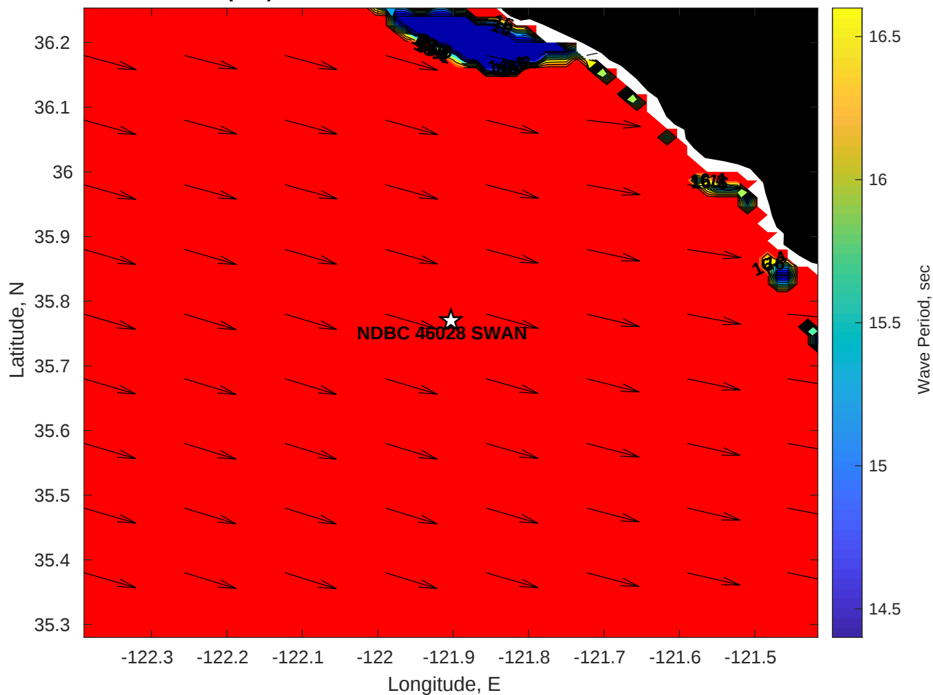
SWAN Wave Period (sec) for NDBC 46028 SWAN at 03-Dec-2025 10:00:00
