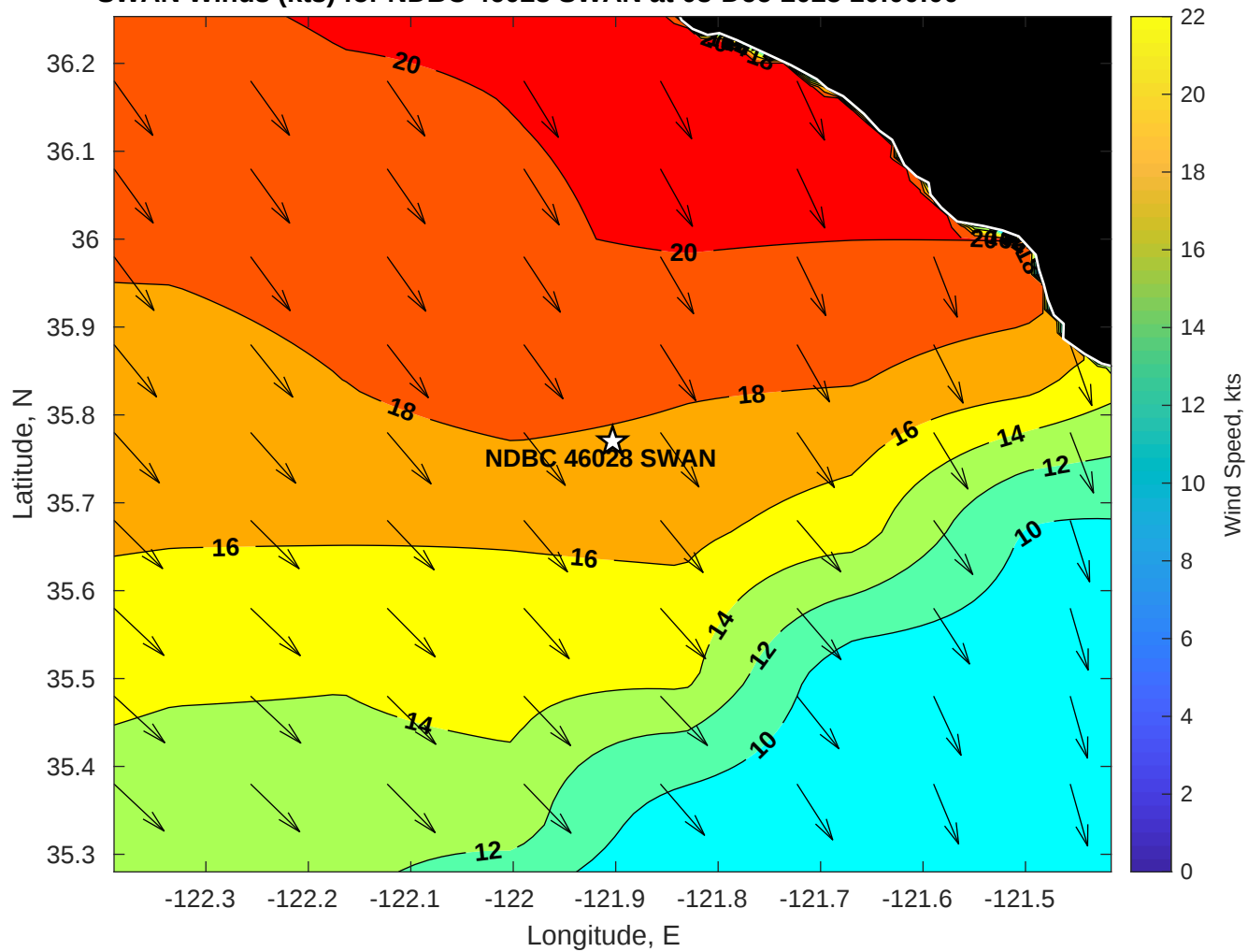
SWAN Winds (kts) for NDBC 46028 SWAN at 03-Dec-2025 10:00:00
