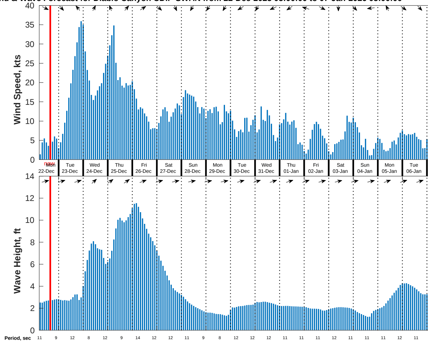
Wind & Wave Forecast for Diablo Canyon CDIP SWAN from 22-Dec-2025 05:00:00 to 07-Jan-2026 05:00:00
