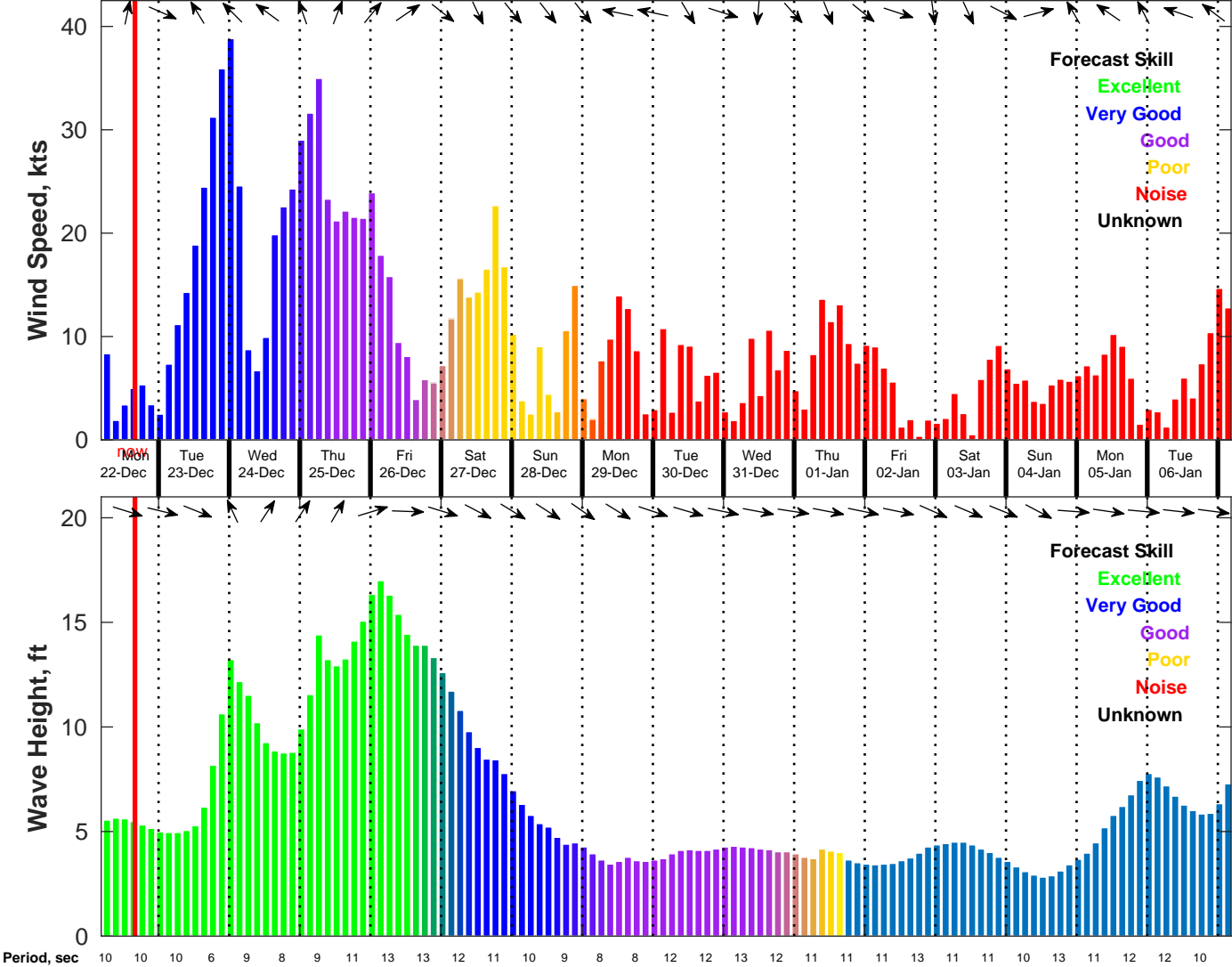
Wind & Wave Forecast for NDBC 46028 GFS from 22-Dec-2025 05:00:00 to 07-Jan-2026 05:00:00
