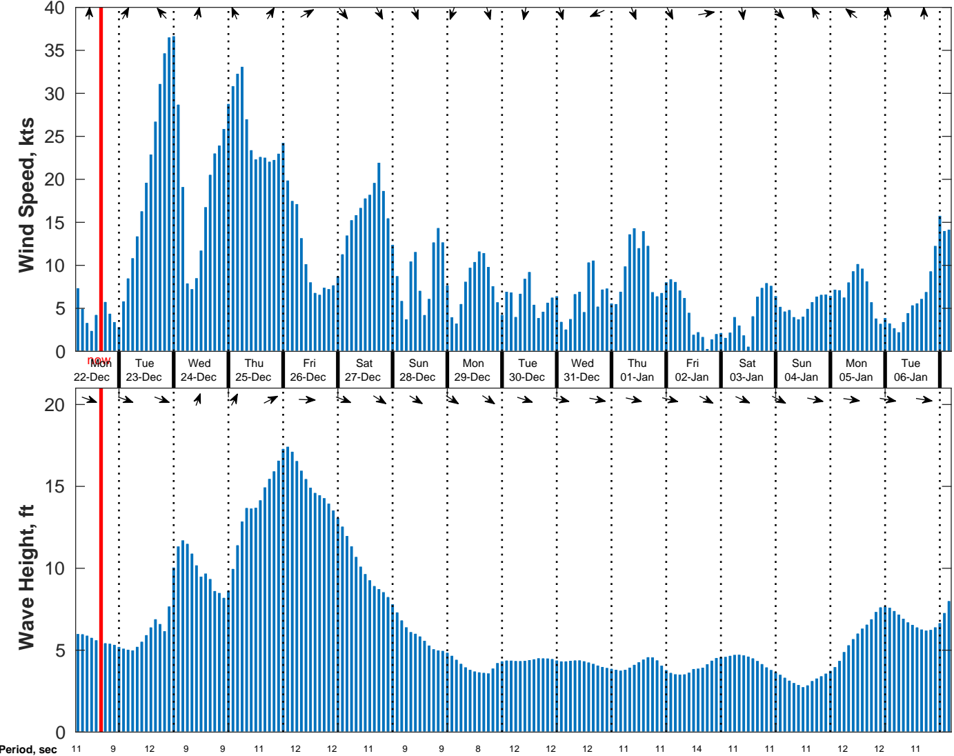
Wind & Wave Forecast for NDBC 46028 SWAN from 22-Dec-2025 05:00:00 to 07-Jan-2026 05:00:00
