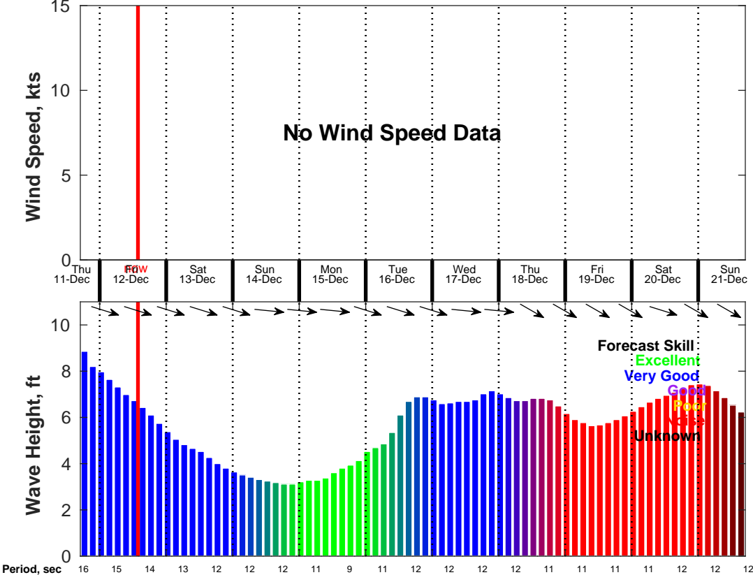
Wind & Wave Forecast for NDBC 46011 from 11-Dec-2025 17:00:00 to 21-Dec-2025 17:00:00
