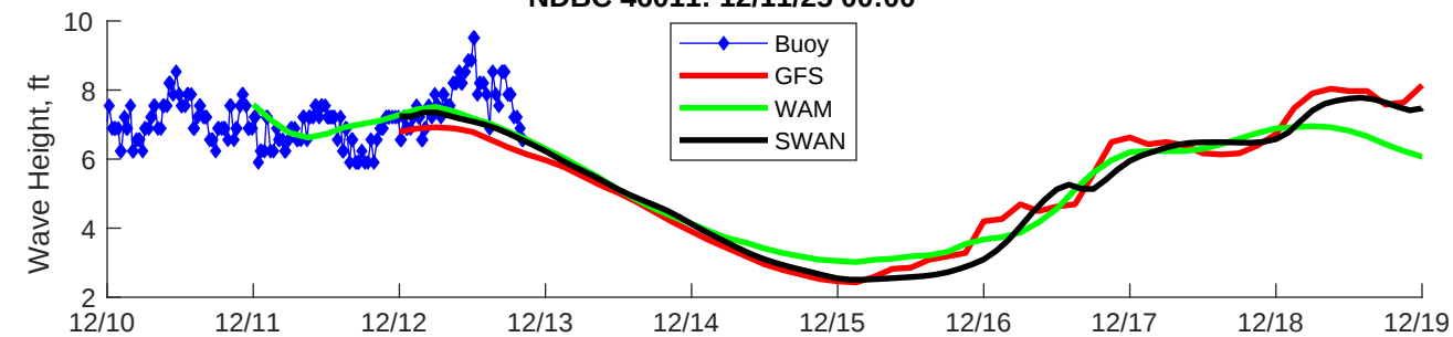
NDBC 46011: 12/11/25 00:00
