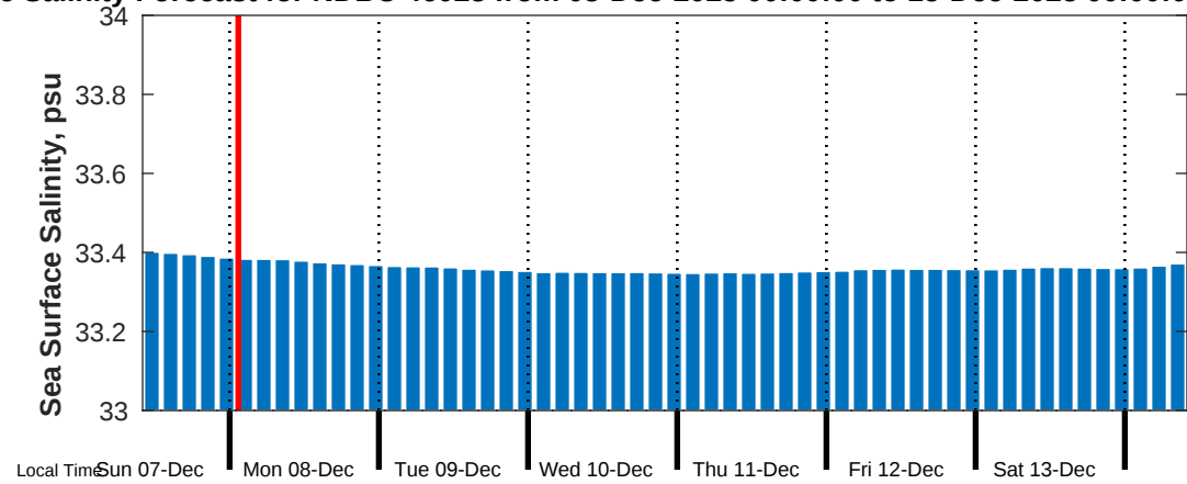
Sea Surface Salinity Forecast for NDBC 46028 from 08-Dec-2025 00:00:00 to 15-Dec-2025 00:00:00
