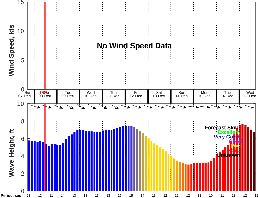
Wind & Wave Forecast for NDBC 46028 from 07-Dec-2025 17:00:00 to 17-Dec-2025 17:00:00
