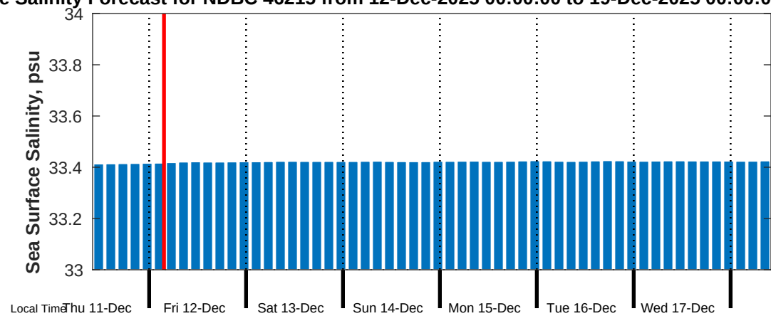
Sea Surface Salinity Forecast for NDBC 46215 from 12-Dec-2025 00:00:00 to 19-Dec-2025 00:00:00
