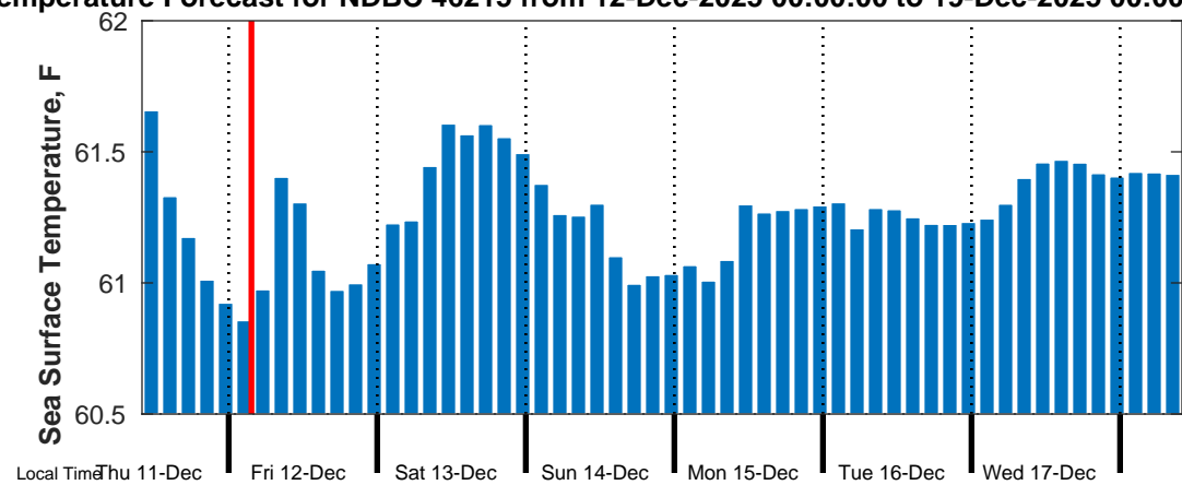
Sea Surface Temperature Forecast for NDBC 46215 from 12-Dec-2025 00:00:00 to 19-Dec-2025 00:00:00
