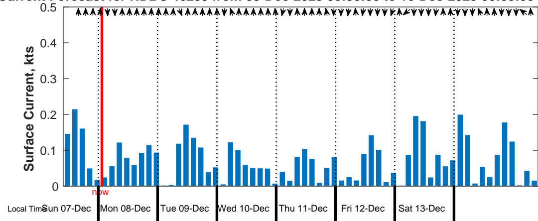
Surface Current Forecast for NDBC 46259 from 08-Dec-2025 00:00:00 to 16-Dec-2025 00:00:00
