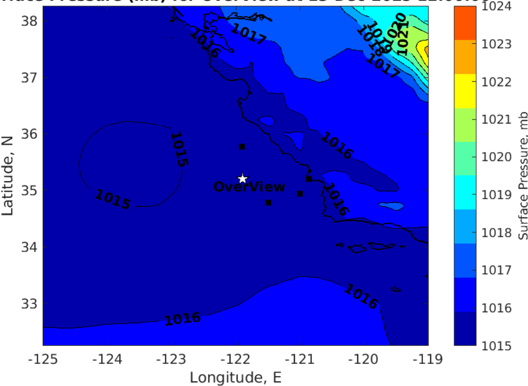
Surface Pressure (mb) for OverView at 13-Dec-2025 12:00:00
