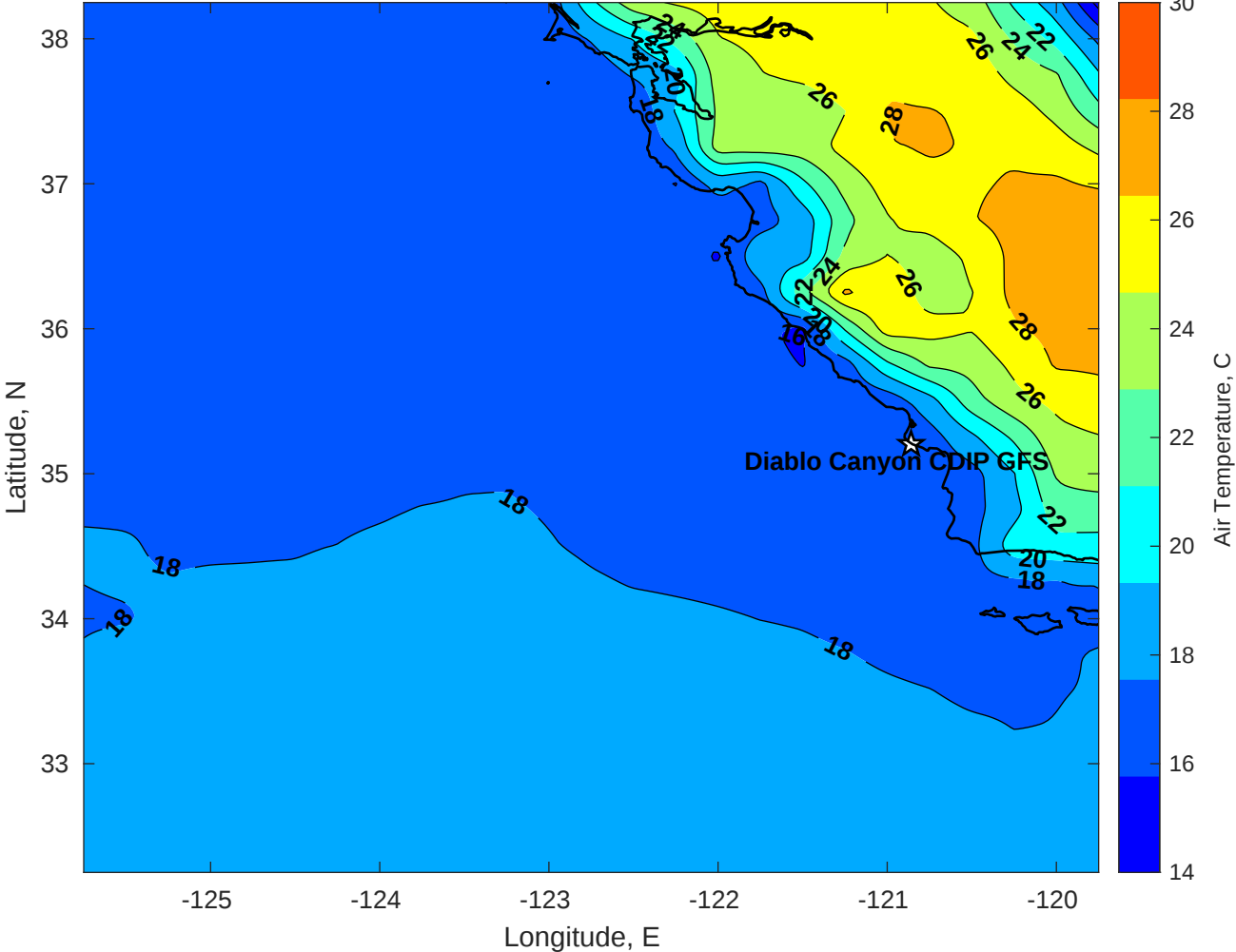
Air Temperature (C) for Diablo Canyon CDIP GFS at 22-Oct-2025
