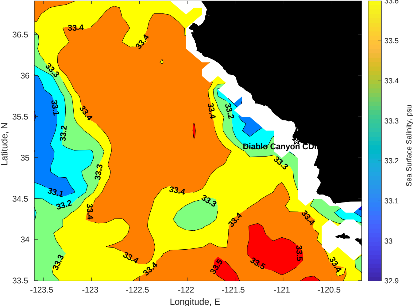
Surface Salinity for Diablo Canyon CDIP GFS at 16-Nov-2025 00:00:00
