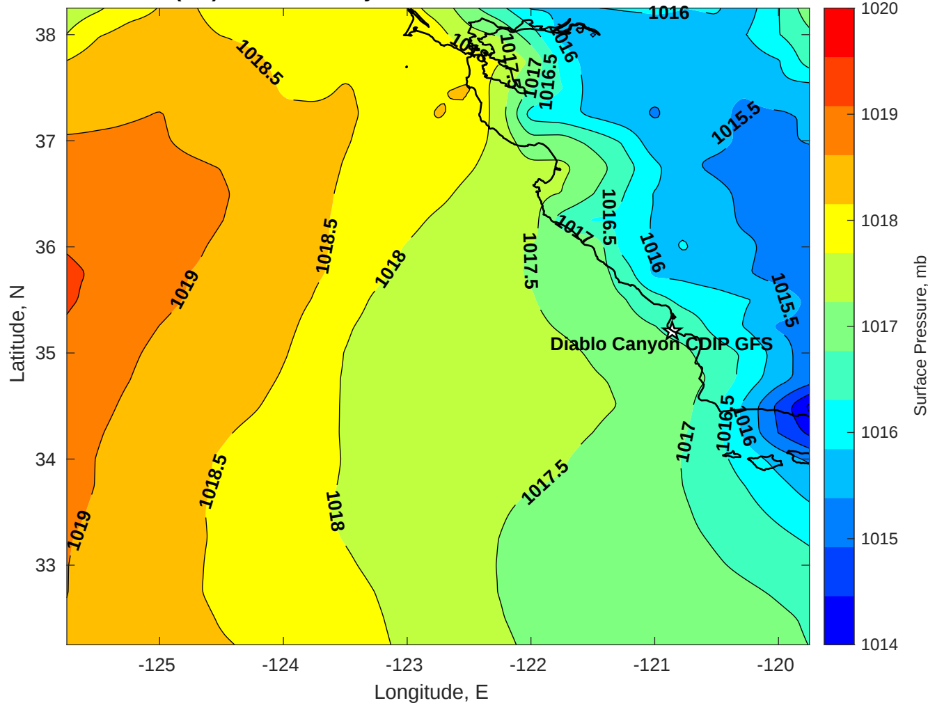
Surface Pressure (mb) for Diablo Canyon CDIP GFS at 23-Oct-2025 00:00:00
