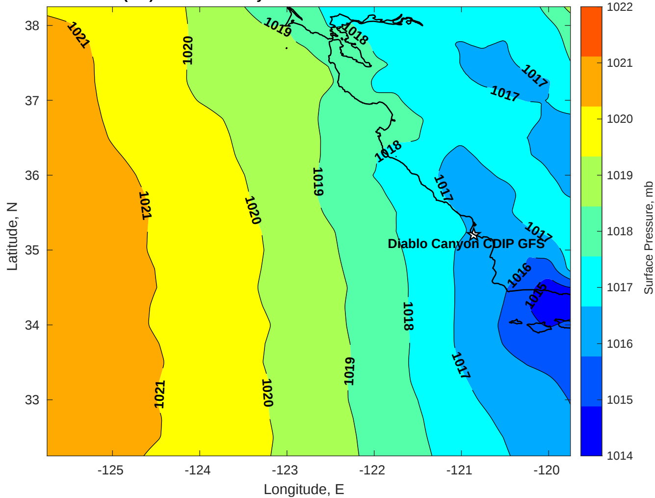
Surface Pressure (mb) for Diablo Canyon CDIP GFS at 24-Oct-2025 00:00:00
