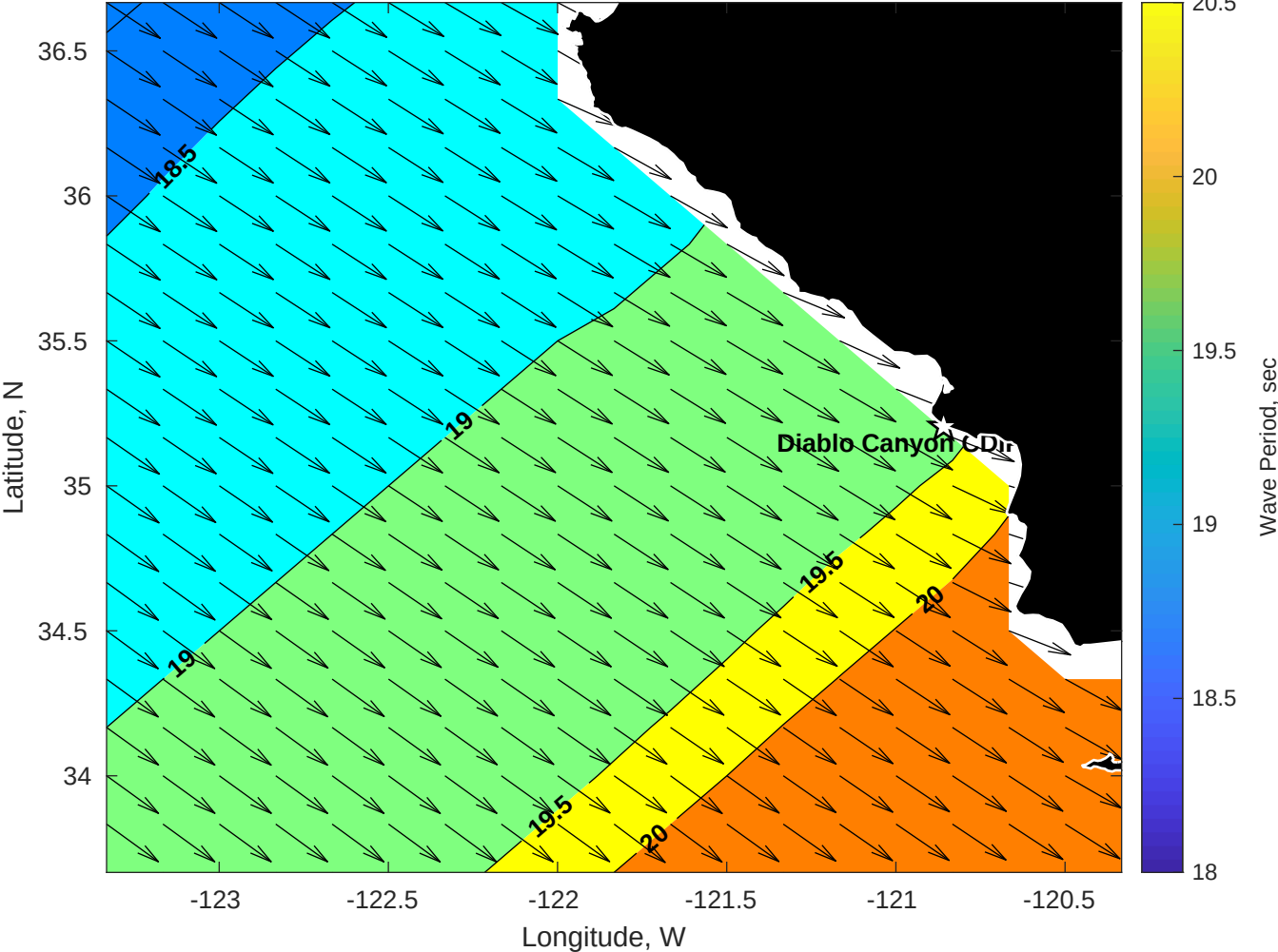
Wave Period (sec) for Diablo Canyon CDIP GFS at 22-Oct-2025 09:00:00
