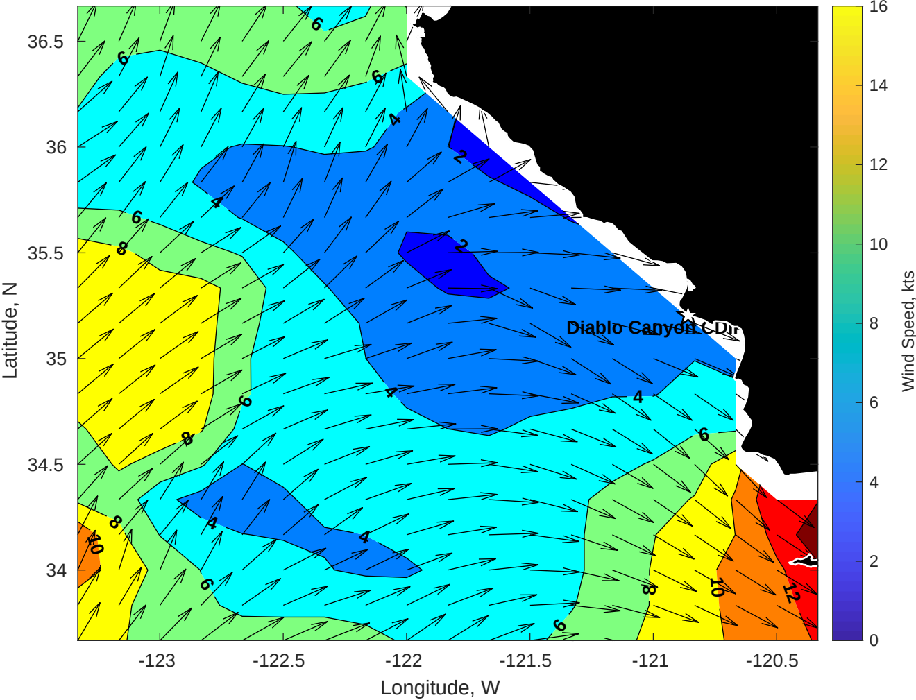
Winds (kts) for Diablo Canyon CDIP GFS at 22-Oct-2025 09:00:00
