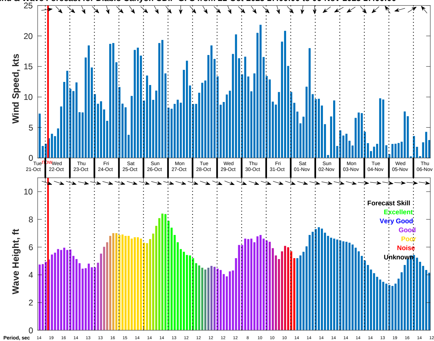
Wind & Wave Forecast for Diablo Canyon CDIP GFS from 21-Oct-2025 17:00:00 to 06-Nov-2025 17:00:00
