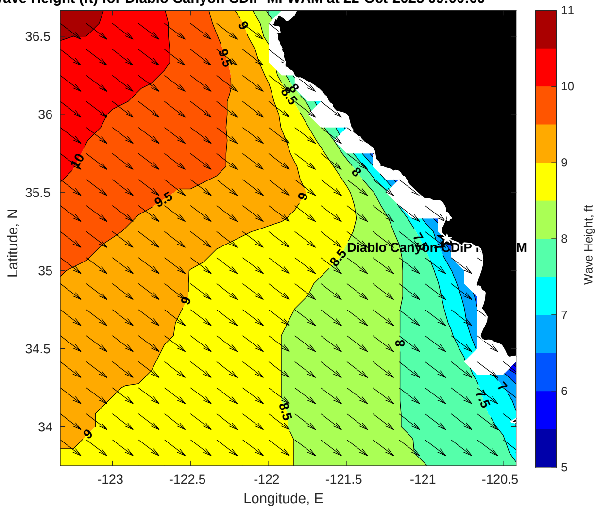
Wave Height (ft) for Diablo Canyon CDIP MFWAM at 22-Oct-2025 09:00:00
