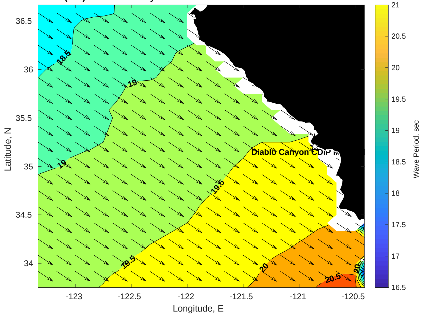
Wave Period (sec) for Diablo Canyon CDIP MFWAM at 22-Oct-2025 09:00:00
